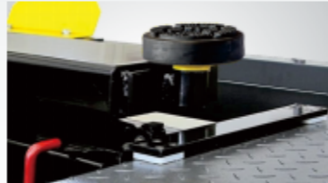
Extendable lower sliding assembly with plastic sliders that support the easy, smooth movement of the jack.
