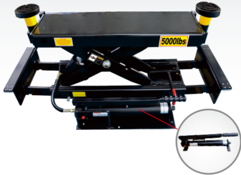
The commercial-grade manual pump is easy to use and requires no additional air source
