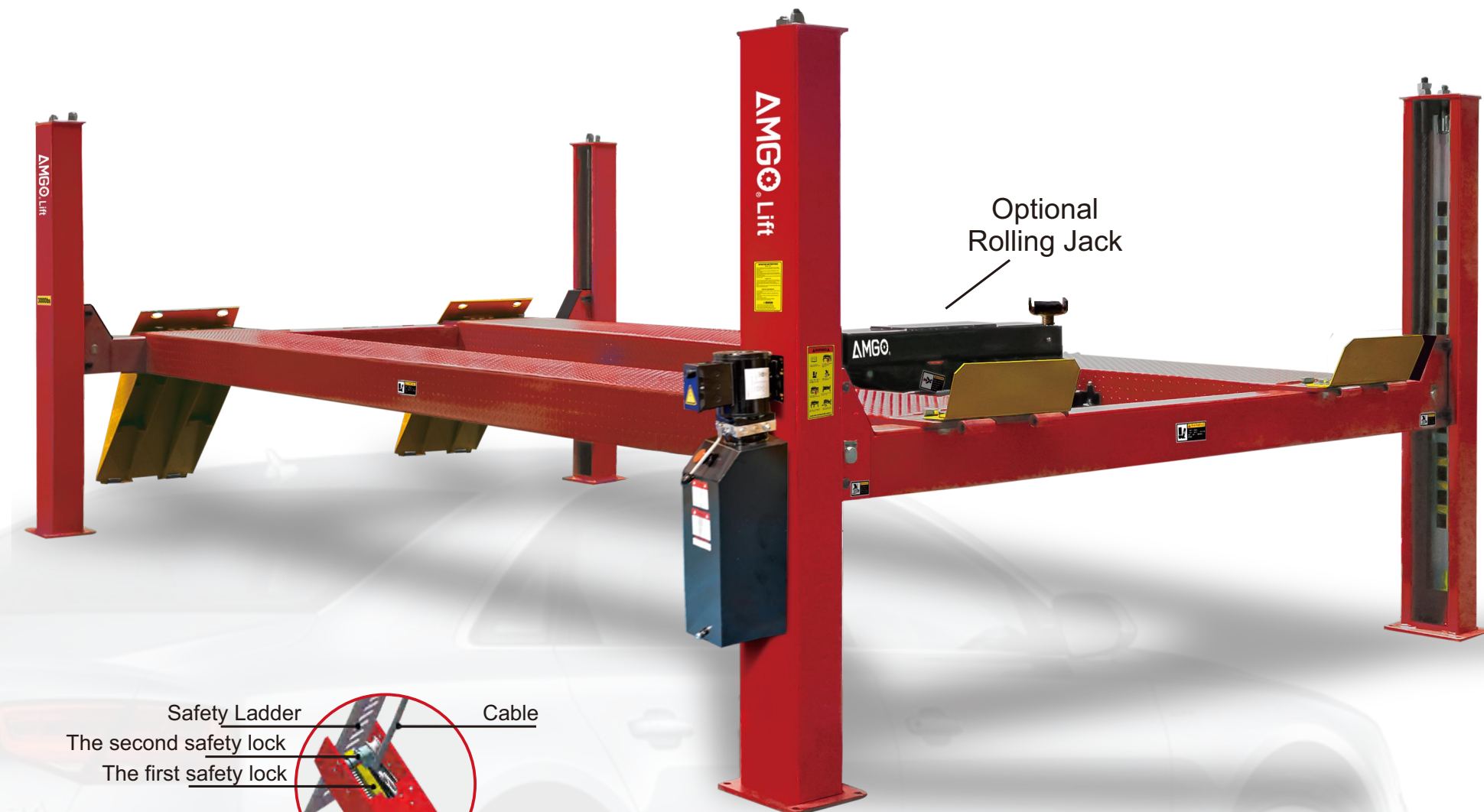
Double-safety locks
