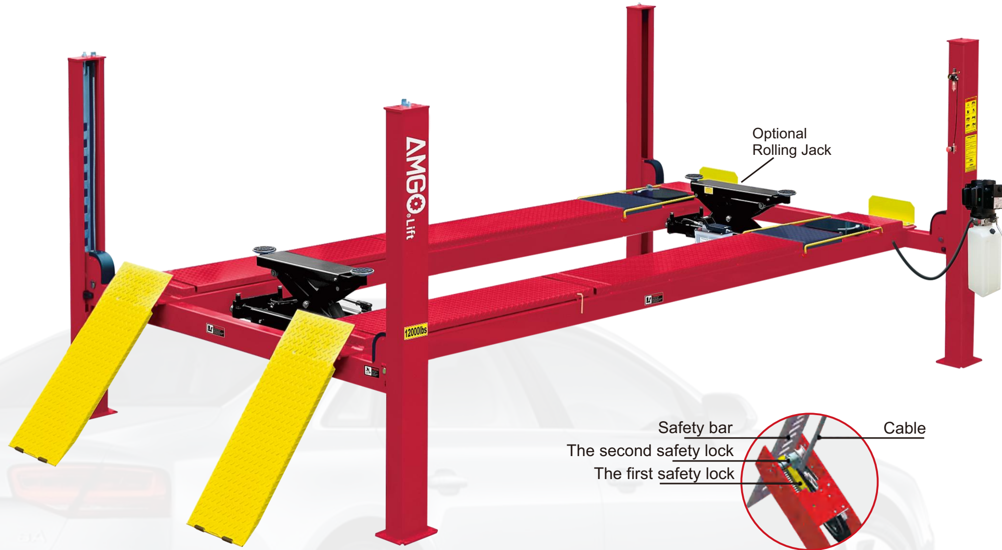
Double-safety locks
