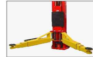
Three-stages Arms The OH-12 OH-12S with 4 three-stages arms allowing to lift the trucks from short to long wheel base.
