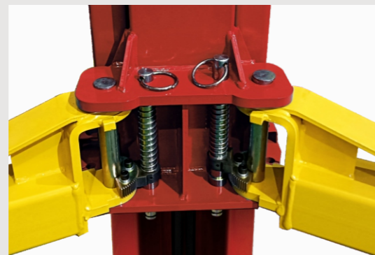
• Lifting arms lock automatic release device, high strength gear rack, more stable and reliable.
