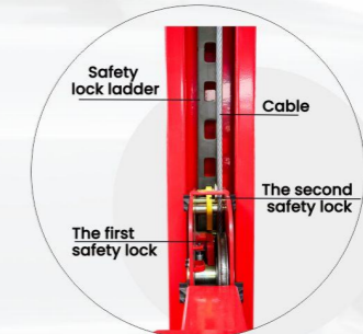
Double-safety locks
