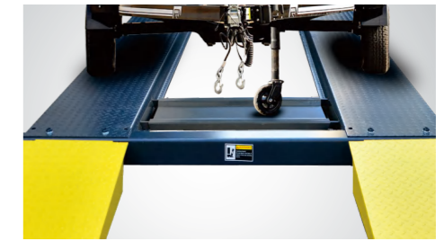
Standard adjustable trailer platform. Adj. range: 42 3/8"-66 1/4".
