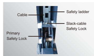
Double safety locks provide additional safety.
