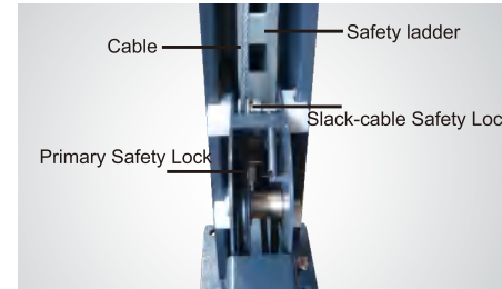
Double safety locks provide additional safety.
